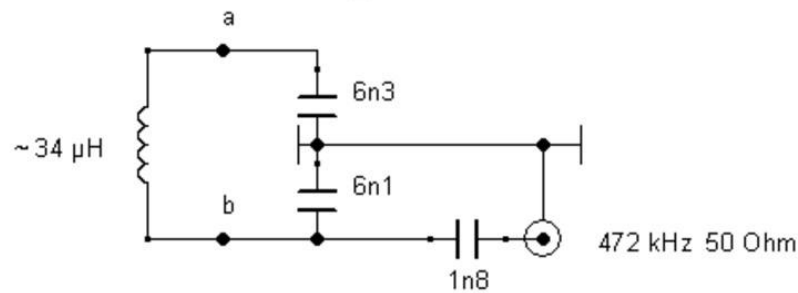
Measured values @ 472 kHz
