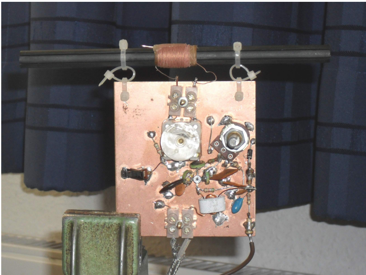
Test circuit: Preamplifier with 500 kHz ferrite rod antenna
