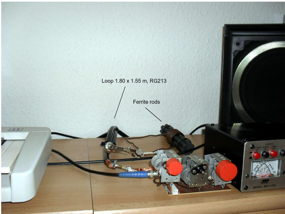
Ferrite rod / loop antenna test circuit
